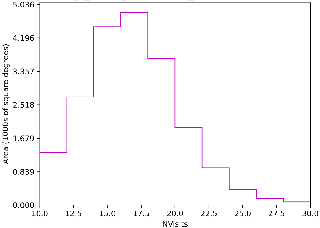
internal_u_expt30_nscale1.5v3.4_10yrs Yr 1 z band: NVisits
