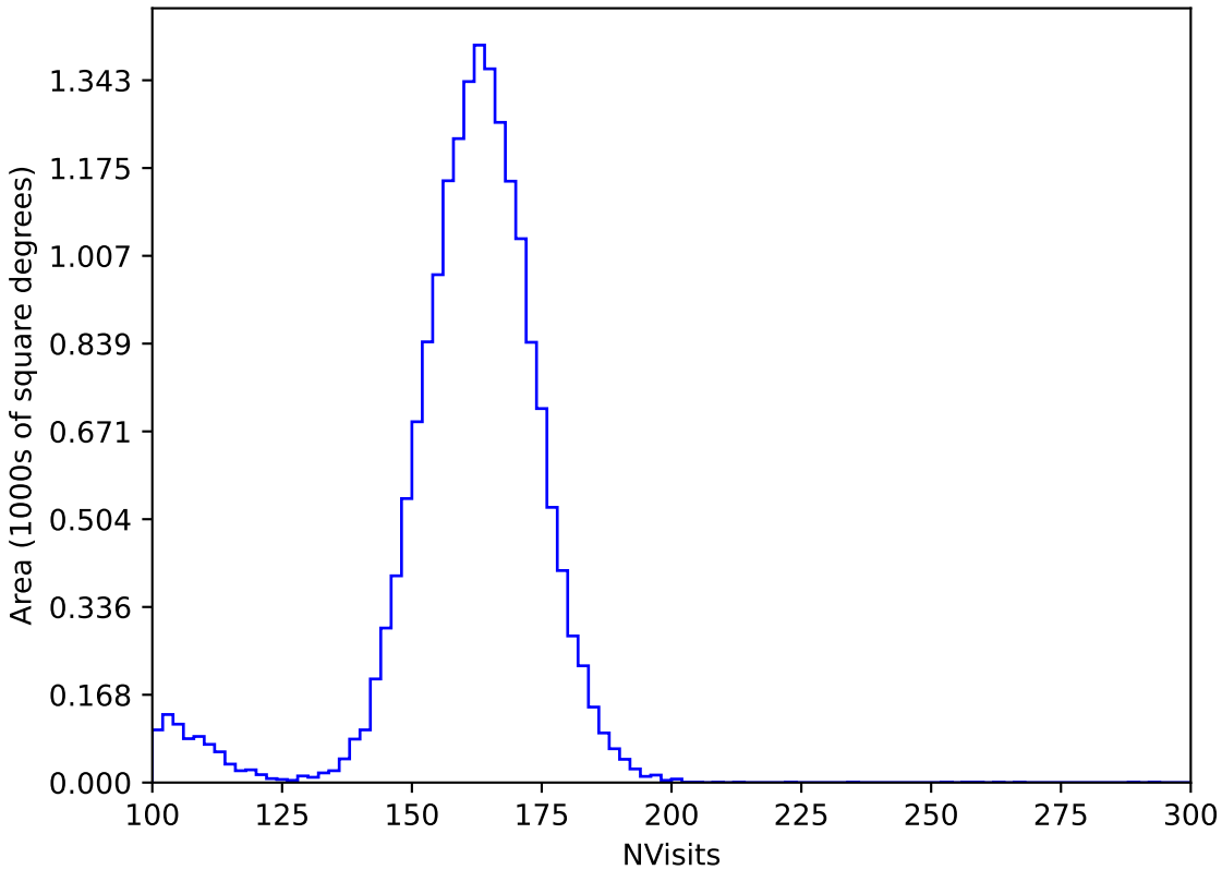
internal_u_expt30_nscale1.5v3.4_10yrs WFD y band: NVisits
