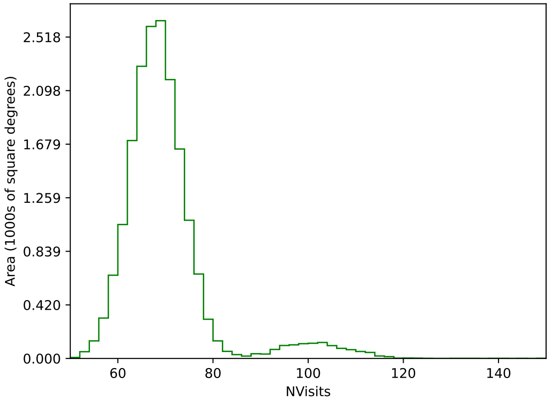
internal_u_expt30_nscale1.5v3.4_10yrs WFD g band: NVisits
