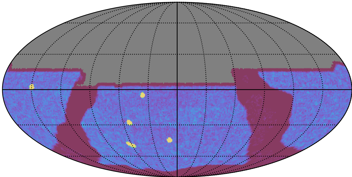
internal_u_expt30_nscale1.5v3.4_10yrs All sky y band: NVisits
