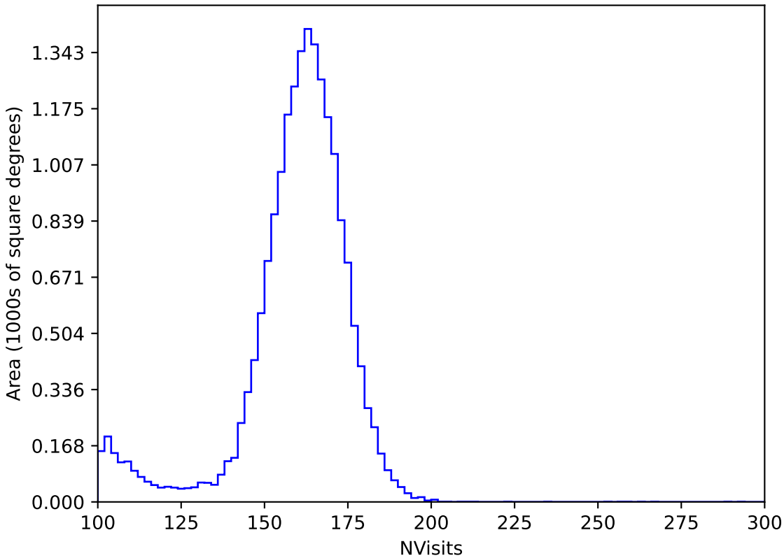
internal_u_expt30_nscale1.5v3.4_10yrs All sky y band: NVisits
