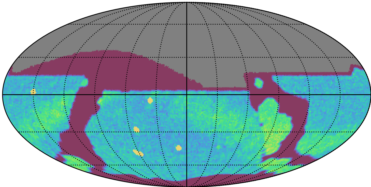
internal_u_expt30_nscale1.5v3.4_10yrs All sky r band: NVisits
