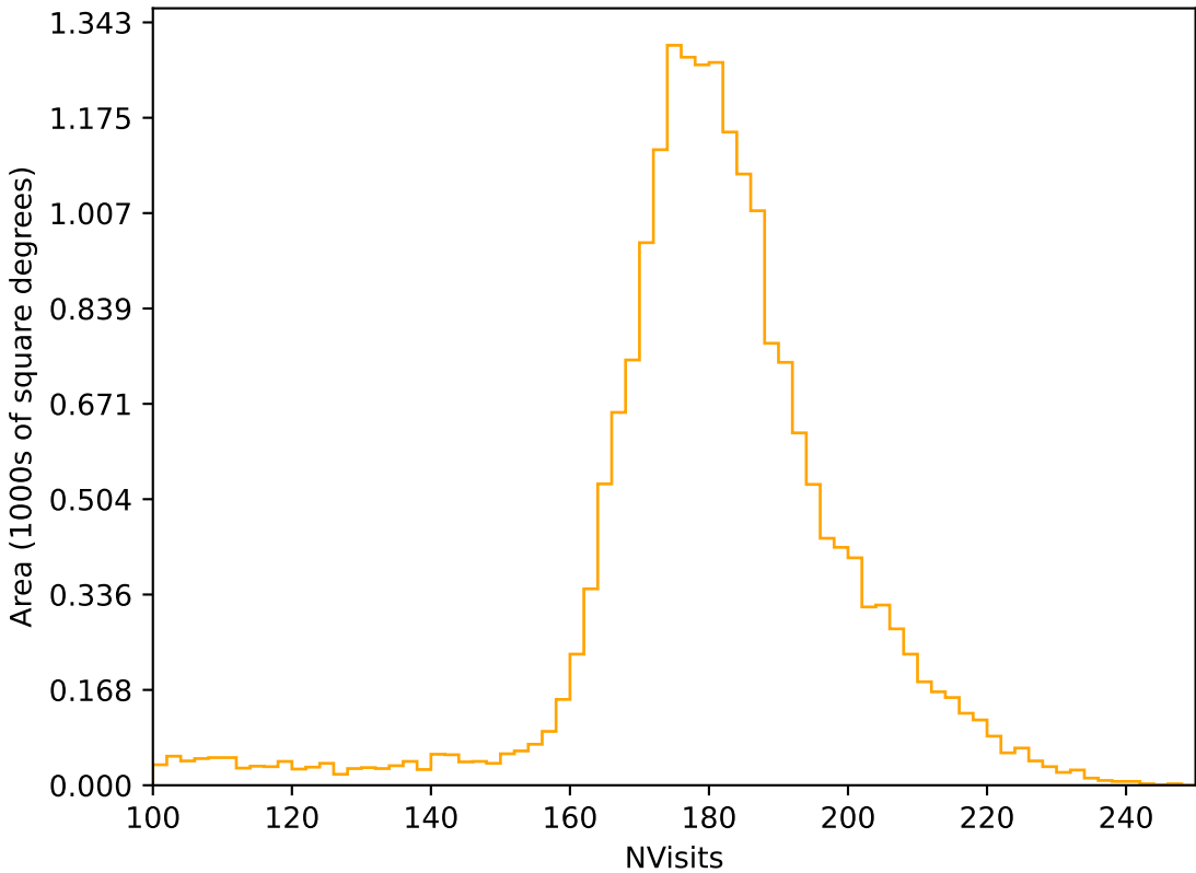
internal_u_expt30_nscale1.5v3.4_10yrs All sky r band: NVisits
