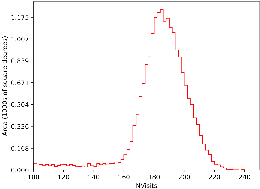
internal_u_expt30_nscale1.5v3.4_10yrs All sky i band: NVisits
