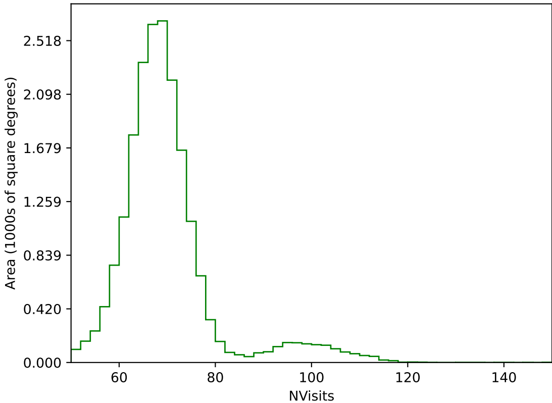
internal_u_expt30_nscale1.5v3.4_10yrs All sky g band: NVisits
