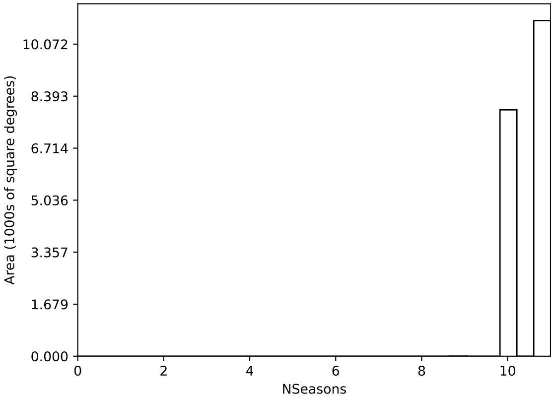
internal_u_expt30_nscale1.5v3.4_10yrs WFD all bands: NSeasons
