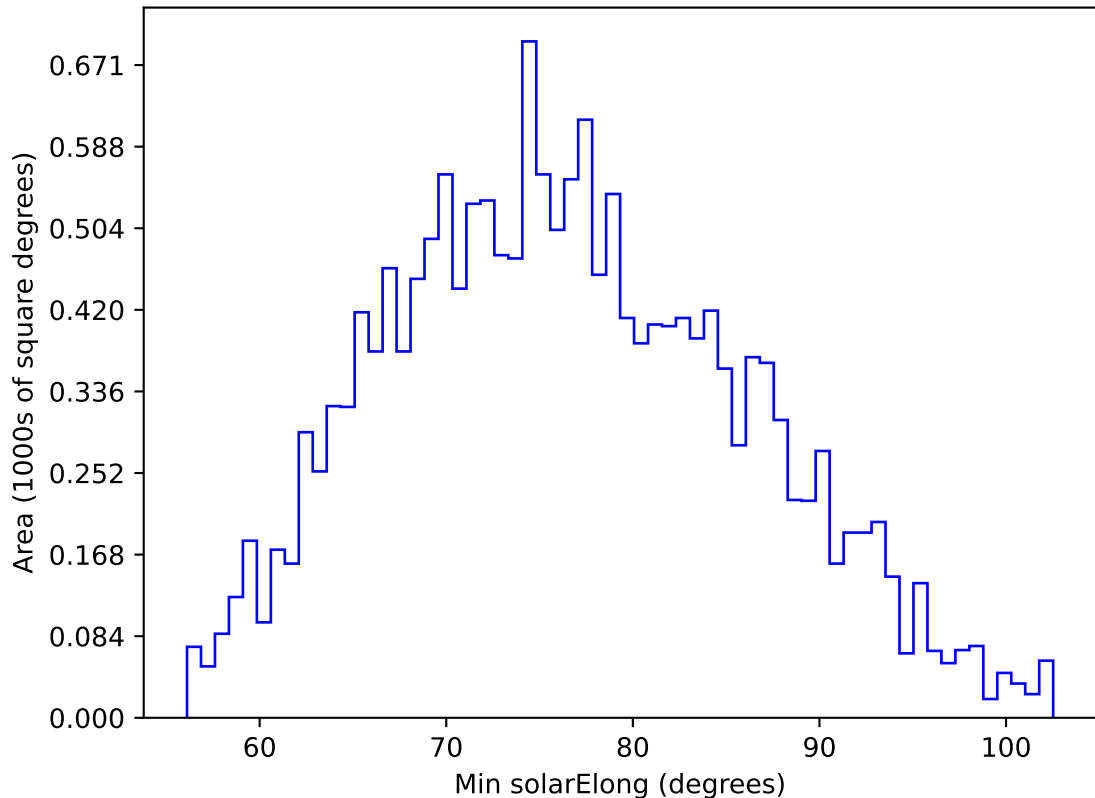
internal_u_expt30_nscale1.5v3.4_10yrs WFD g band: Min solarElong
