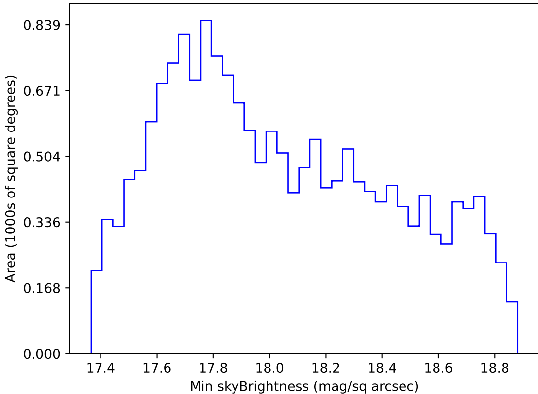
internal_u_expt30_nscale1.5v3.4_10yrs WFD i band: Min skyBrightness
