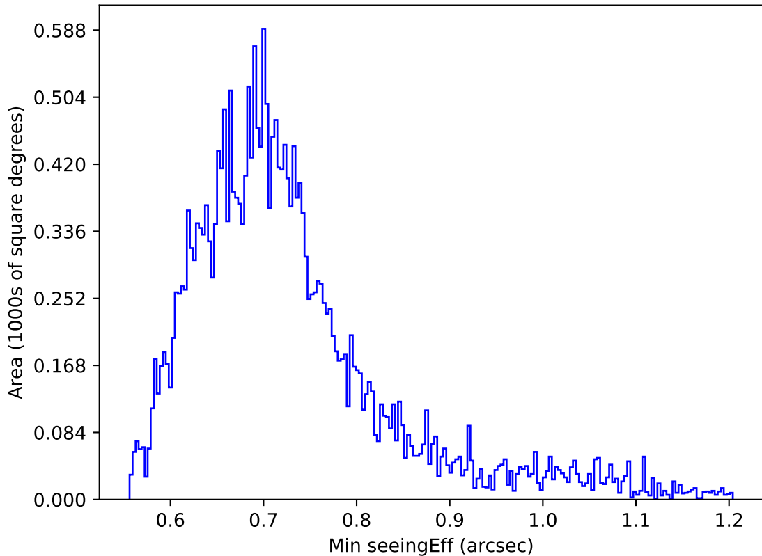
internal_u_expt30_nscale1.5v3.4_10yrs Yr 1 z band: Min seeingEff
