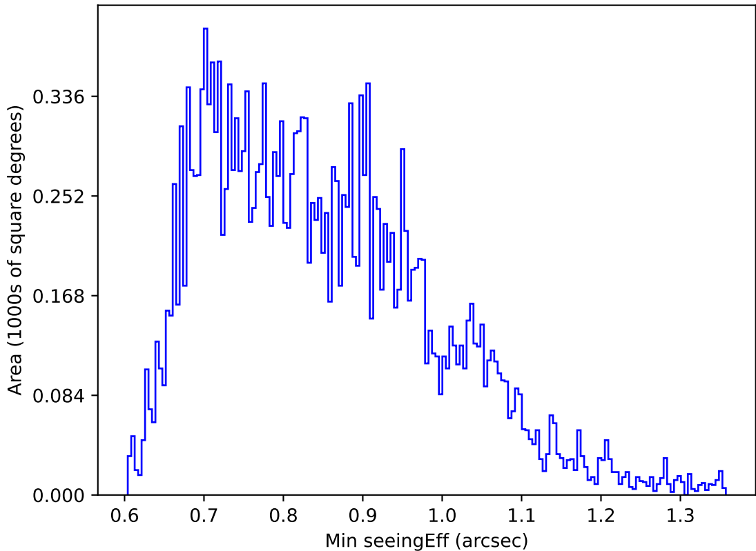
internal_u_expt30_nscale1.5v3.4_10yrs Yr 1 u band: Min seeingEff
