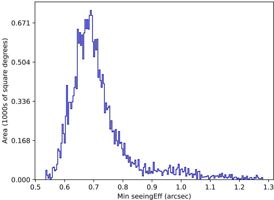
internal_u_expt30_nscale1.5v3.4_10yrs Yr 1 r band: Min seeingEff
