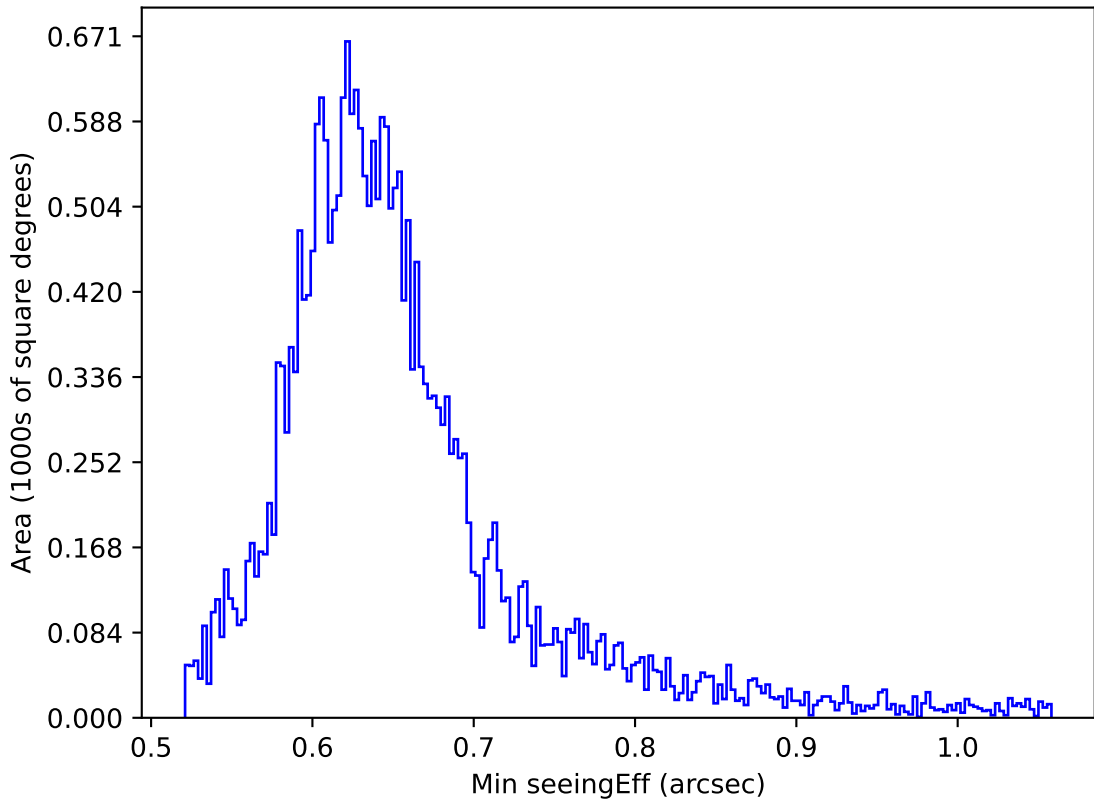
internal_u_expt30_nscale1.5v3.4_10yrs Yr 1 all bands: Min seeingEff
