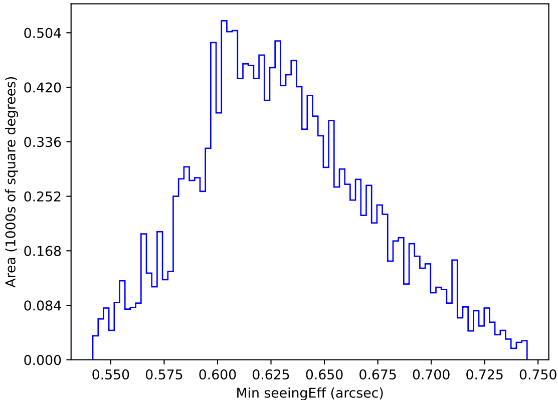
internal_u_expt30_nscale1.5v3.4_10yrs WFD y band: Min seeingEff
