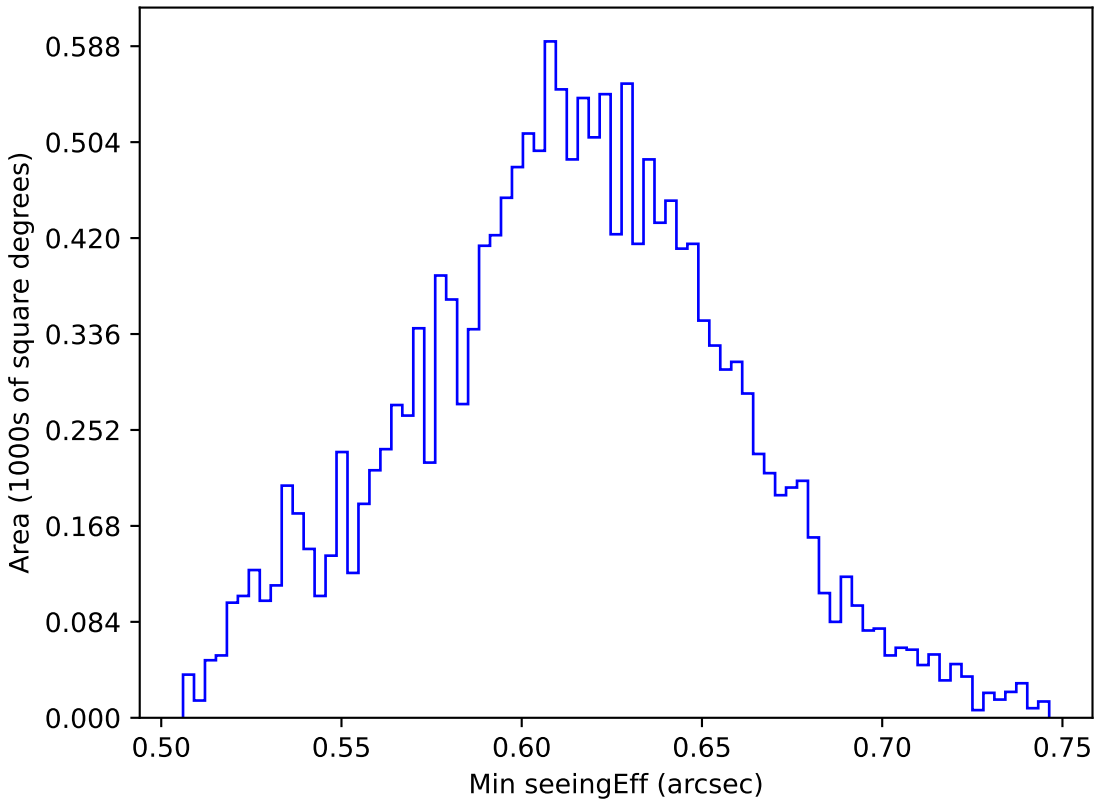
internal_u_expt30_nscale1.5v3.4_10yrs WFD r band: Min seeingEff
