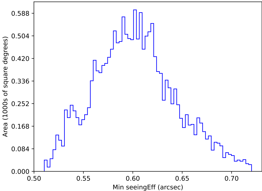
internal_u_expt30_nscale1.5v3.4_10yrs WFD i band: Min seeingEff
