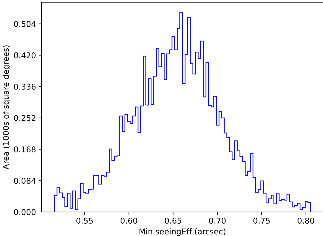
internal_u_expt30_nscale1.5v3.4_10yrs WFD g band: Min seeingEff
