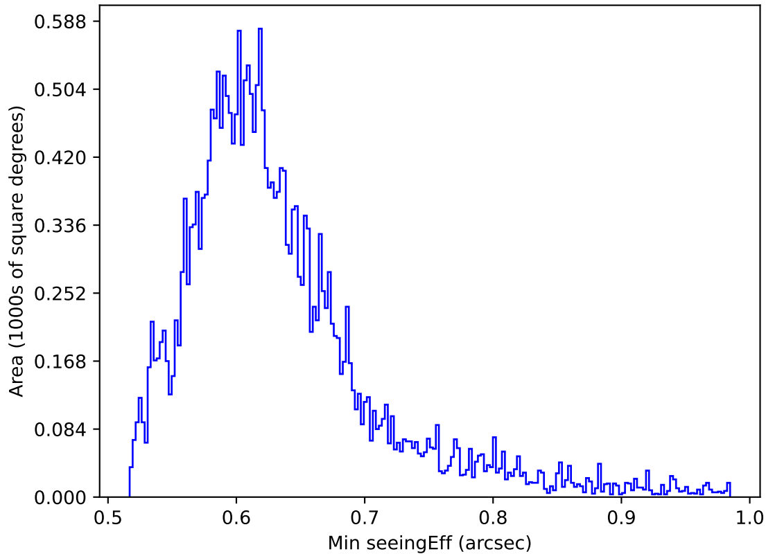
internal_u_expt30_nscale1.5v3.4_10yrs All sky i band: Min seeingEff
