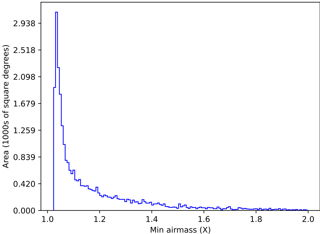
internal_u_expt30_nscale1.5v3.4_10yrs Yr 1 z band: Min airmass
