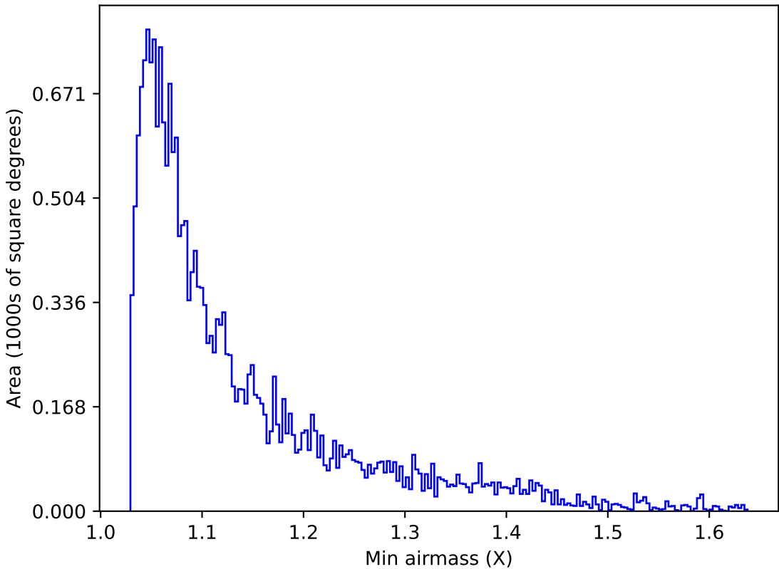
internal_u_expt30_nscale1.5v3.4_10yrs Yr 1 u band: Min airmass
