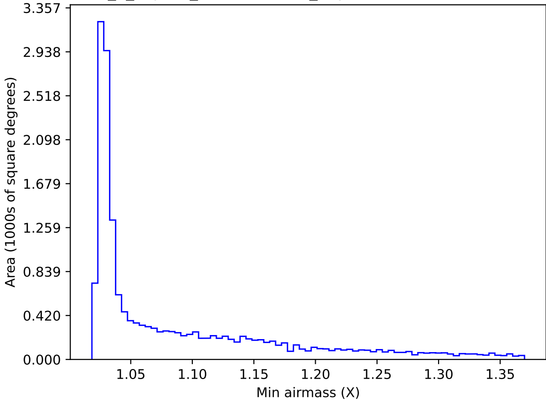
internal_u_expt30_nscale1.5v3.4_10yrs WFD z band: Min airmass
