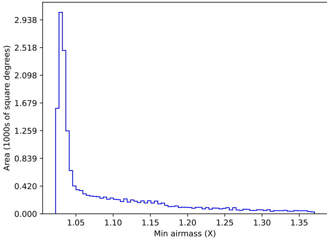
internal_u_expt30_nscale1.5v3.4_10yrs WFD y band: Min airmass
