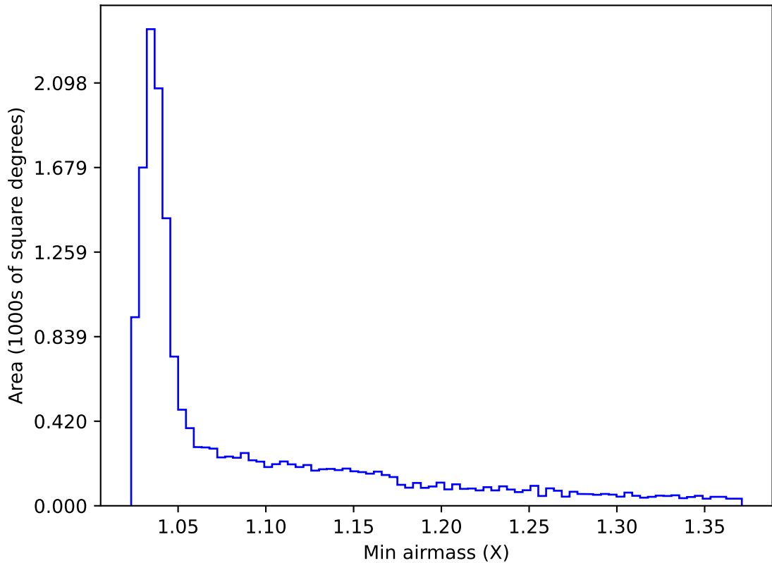
internal_u_expt30_nscale1.5v3.4_10yrs WFD u band: Min airmass
