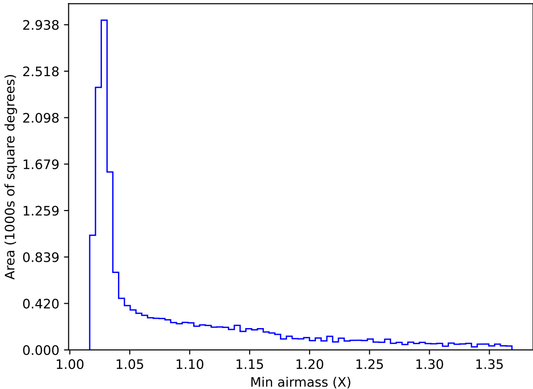
internal_u_expt30_nscale1.5v3.4_10yrs WFD r band: Min airmass
