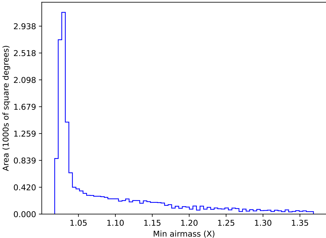
internal_u_expt30_nscale1.5v3.4_10yrs WFD i band: Min airmass
