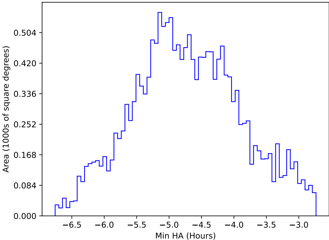
internal_u_expt30_nscale1.5v3.4_10yrs WFD all bands: Min HA
