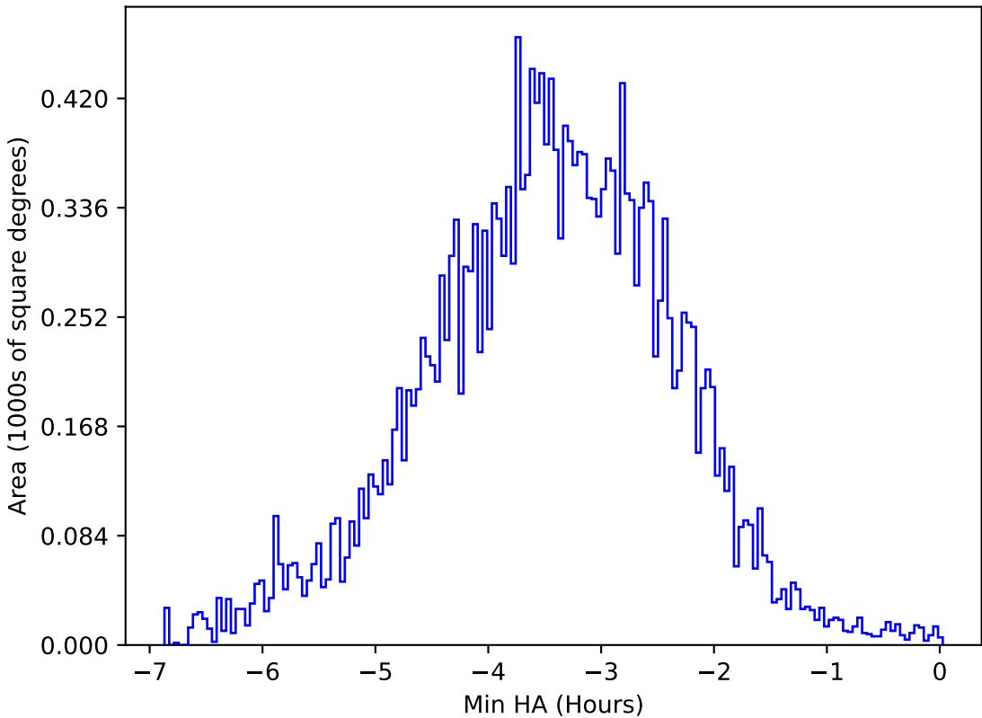
internal_u_expt30_nscale1.5v3.4_10yrs All sky y band: Min HA
