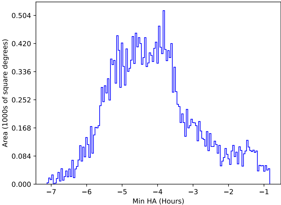
internal_u_expt30_nscale1.5v3.4_10yrs All sky r band: Min HA
