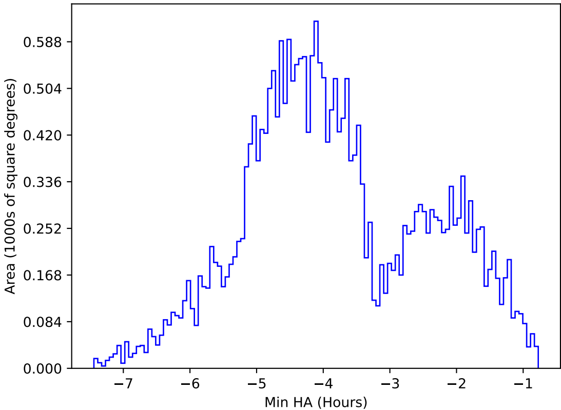
internal_u_expt30_nscale1.5v3.4_10yrs All sky g band: Min HA
