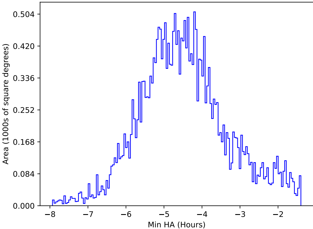
internal_u_expt30_nscale1.5v3.4_10yrs All sky all bands: Min HA
