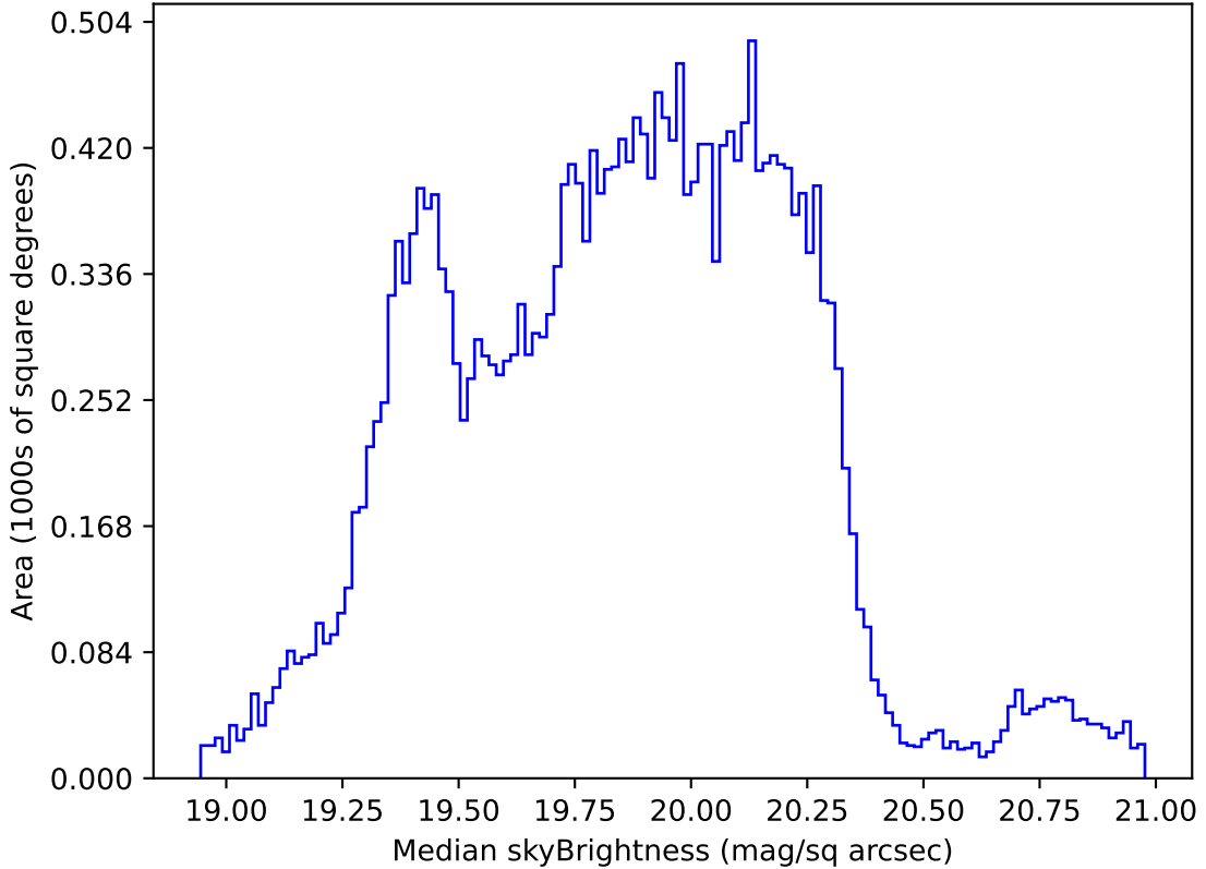
internal_u_expt30_nscale1.5v3.4_10yrs Yr 1 all bands: Median skyBrightness
