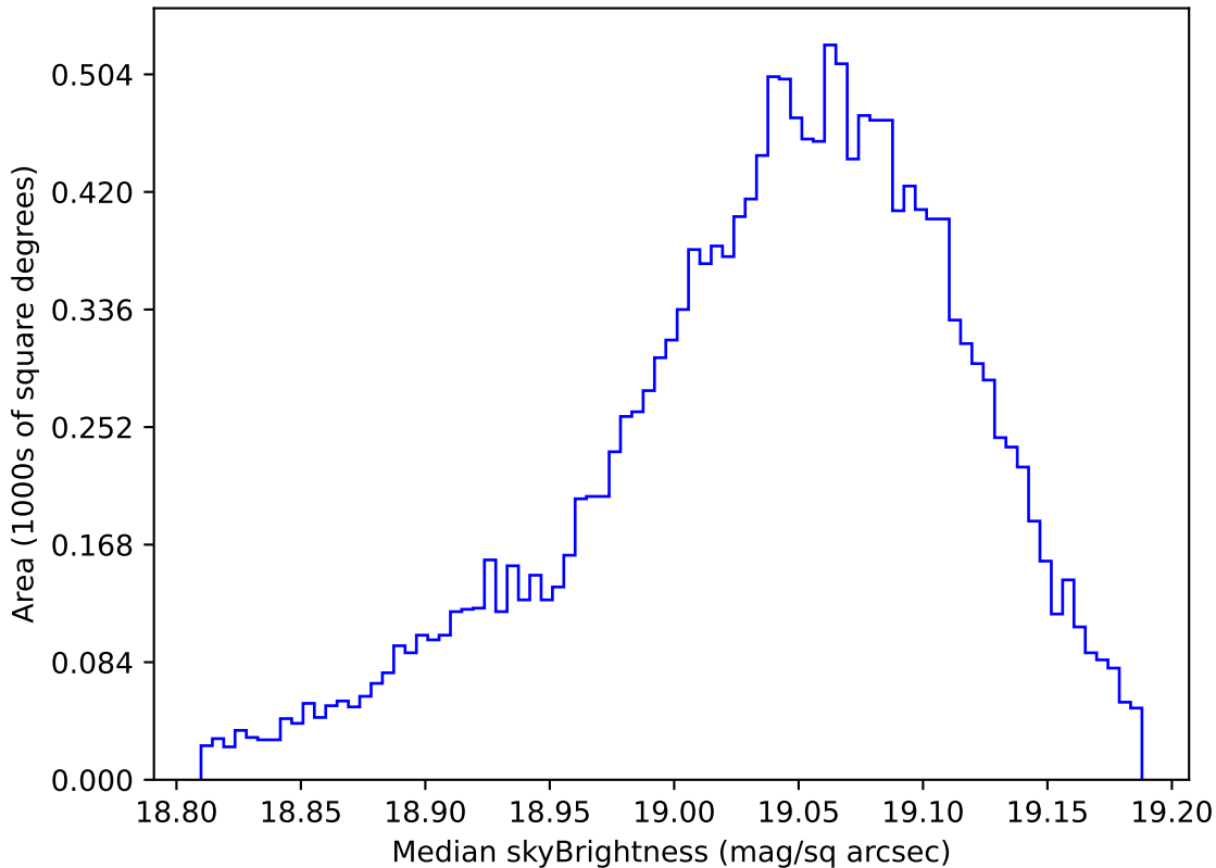
internal_u_expt30_nscale1.5v3.4_10yrs WFD z band: Median skyBrightness
