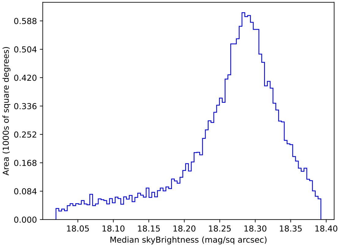
internal_u_expt30_nscale1.5v3.4_10yrs WFD y band: Median skyBrightness
