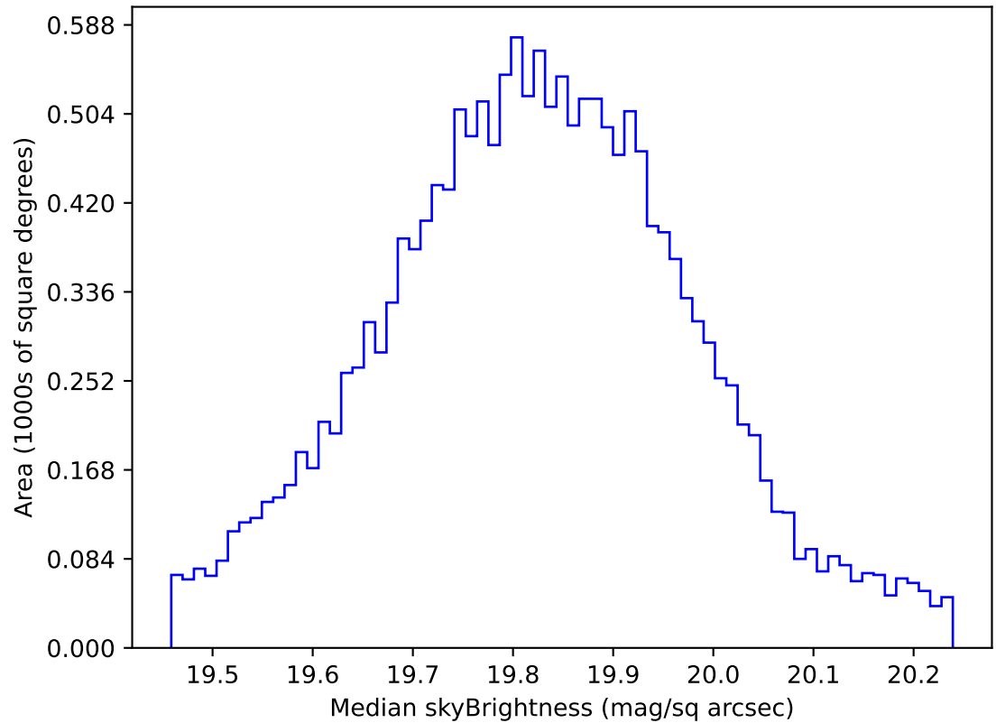
internal_u_expt30_nscale1.5v3.4_10yrs WFD all bands: Median skyBrightness
