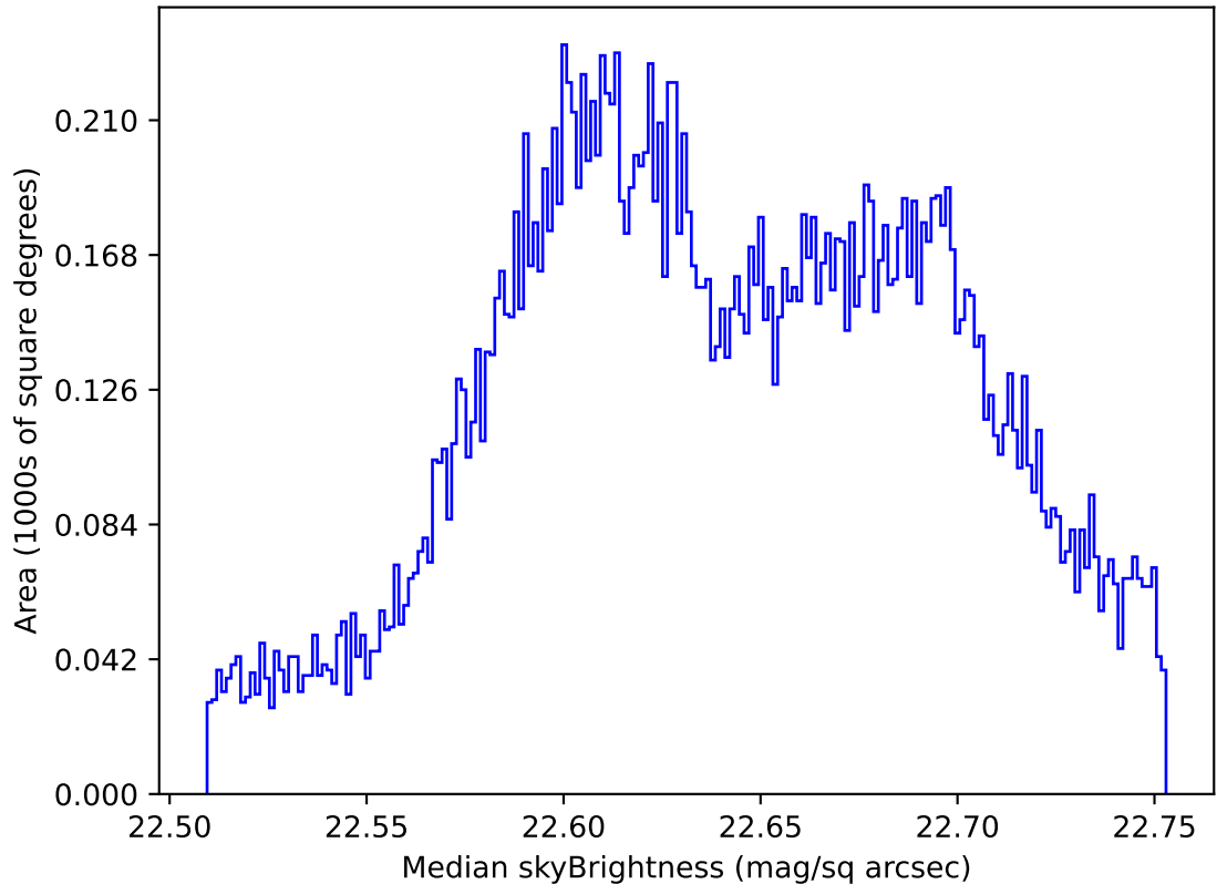
internal_u_expt30_nscale1.5v3.4_10yrs All sky u band: Median skyBrightness
