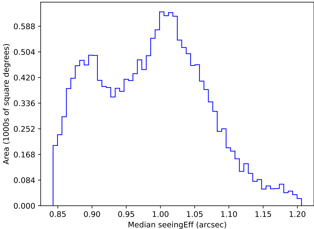
internal_u_expt30_nscale1.5v3.4_10yrs WFD i band: Median seeingEff
