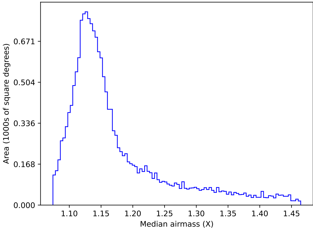
internal_u_expt30_nscale1.5v3.4_10yrs WFD r band: Median airmass
