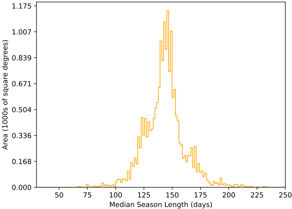
internal_u_expt30_nscale1.5v3.4_10yrs WFD r band: Median Season Length
