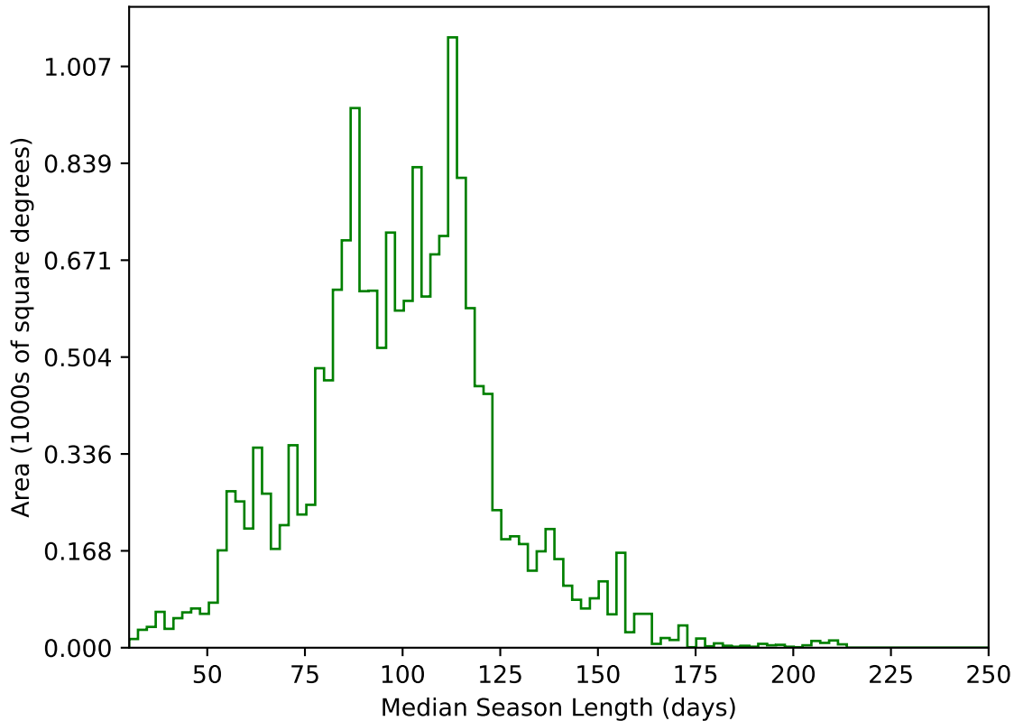
internal_u_expt30_nscale1.5v3.4_10yrs WFD g band: Median Season Length
