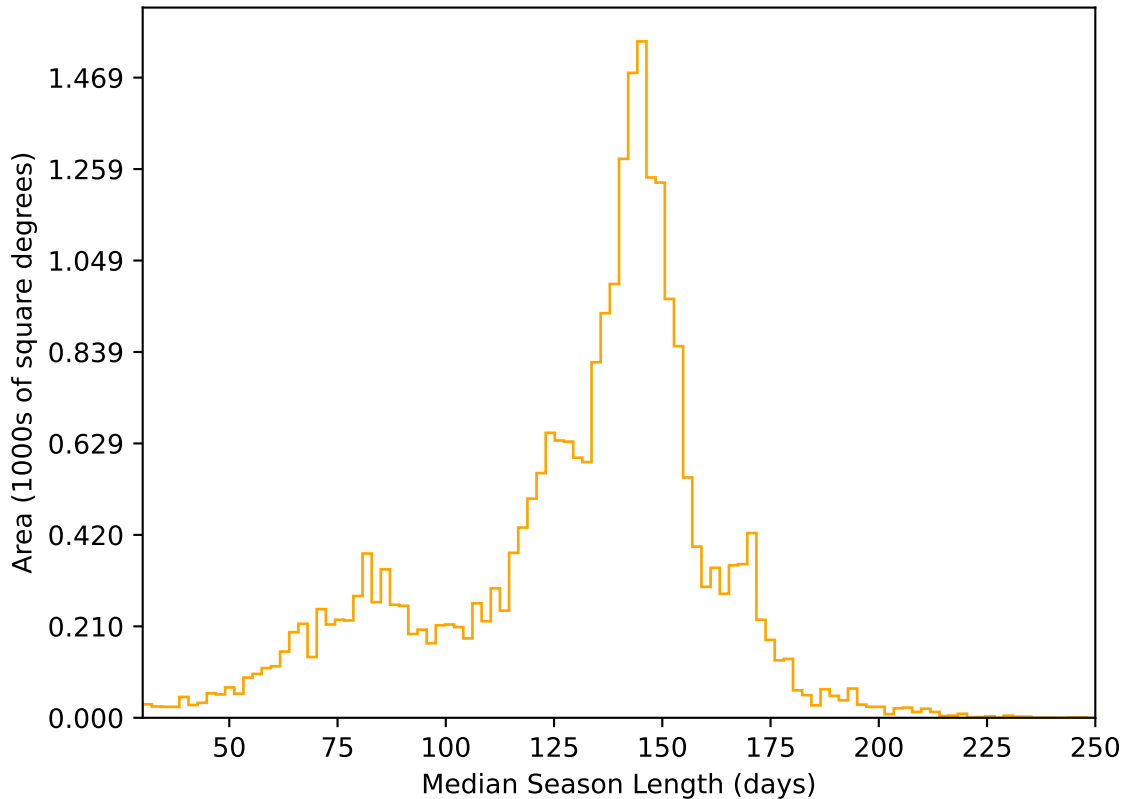
internal_u_expt30_nscale1.5v3.4_10yrs All sky r band: Median Season Length
