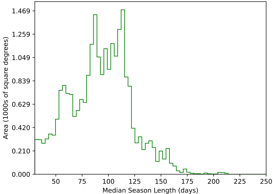
internal_u_expt30_nscale1.5v3.4_10yrs All sky g band: Median Season Length
