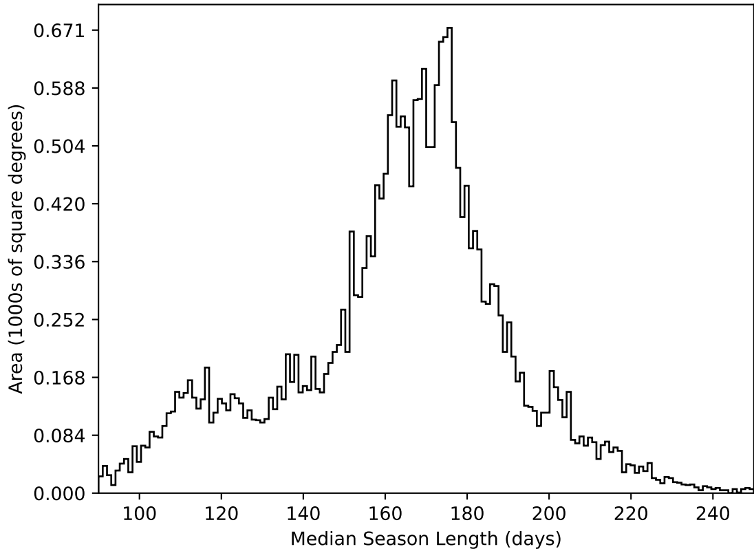
internal_u_expt30_nscale1.5v3.4_10yrs All sky all bands: Median Season Length
