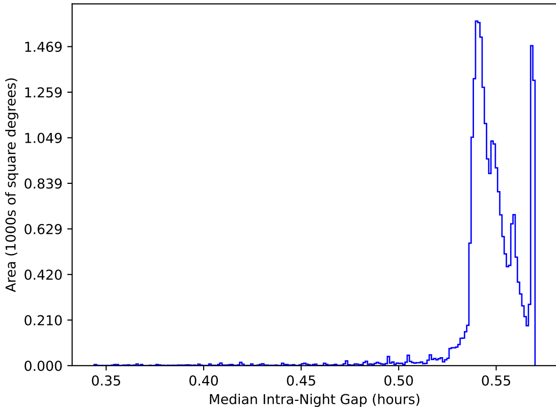
internal_u_expt30_nscale1.5v3.4_10yrs All sky: Median Intra-Night Gap
