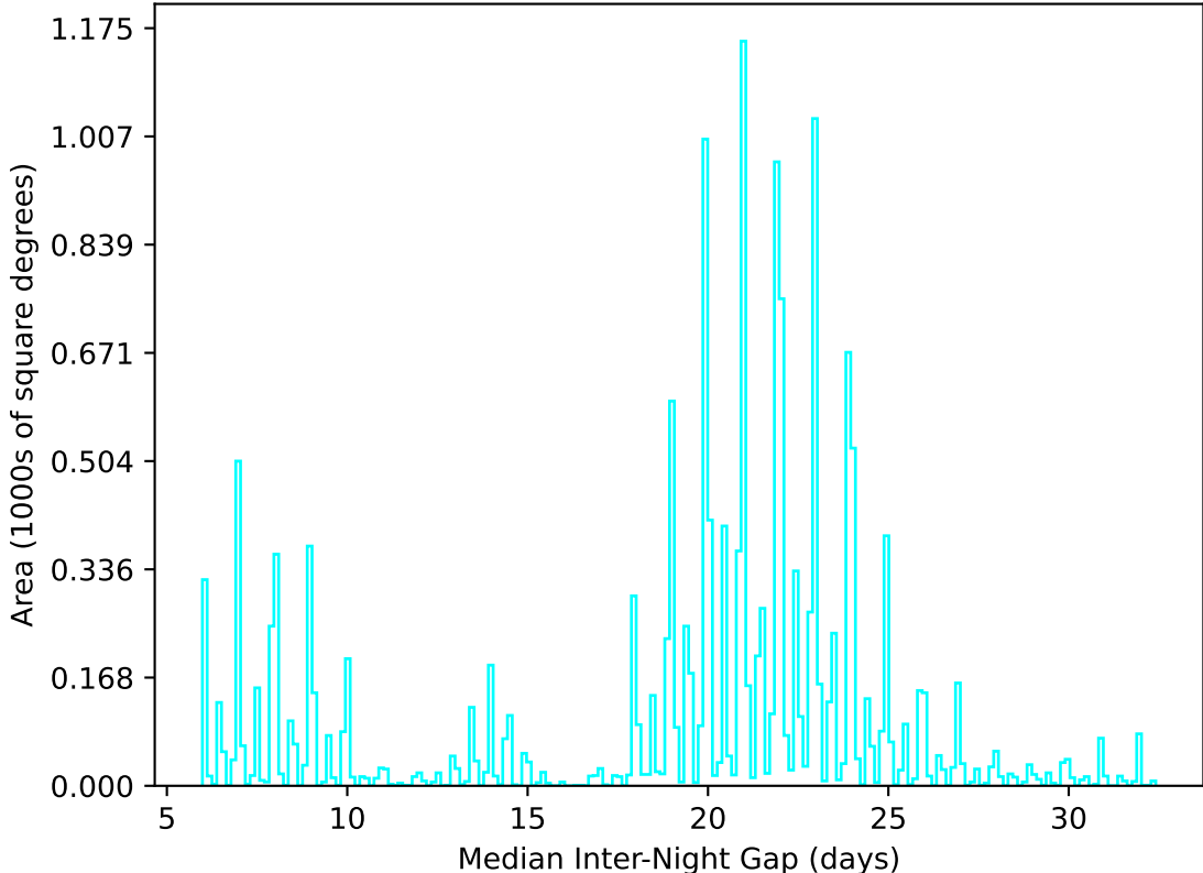
internal_u_expt30_nscale1.5v3.4_10yrs WFD u band: Median Inter-Night Gap
