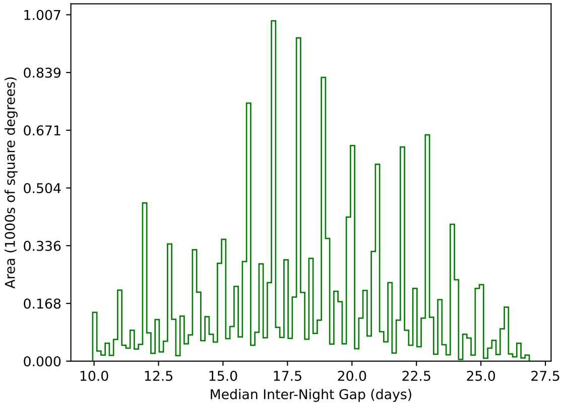
internal_u_expt30_nscale1.5v3.4_10yrs WFD g band: Median Inter-Night Gap
