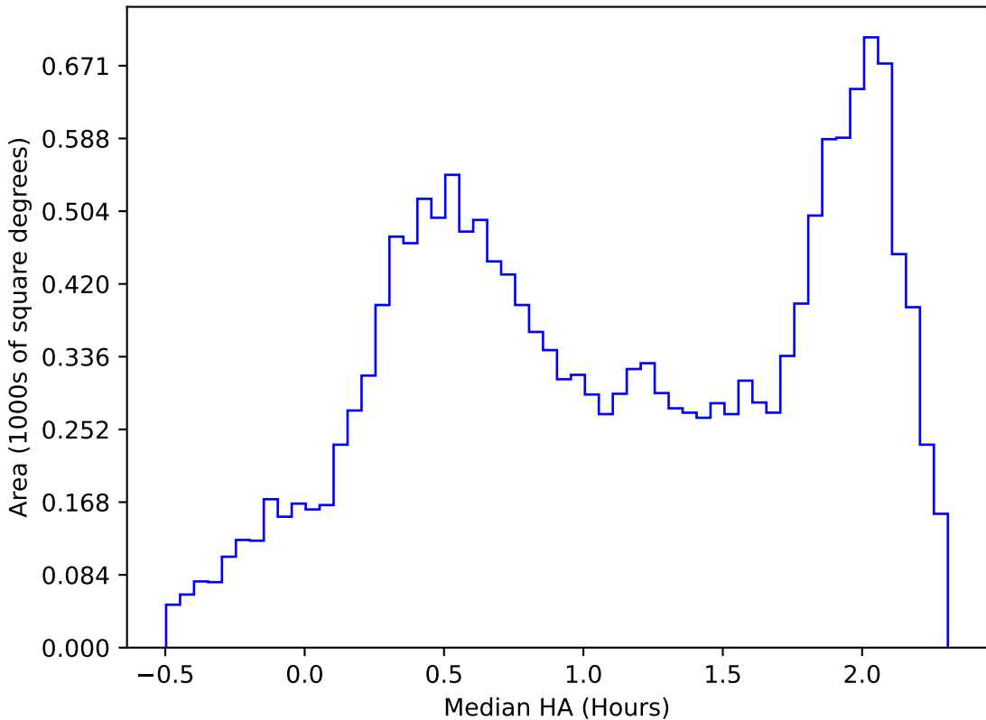
internal_u_expt30_nscale1.5v3.4_10yrs WFD z band: Median HA
