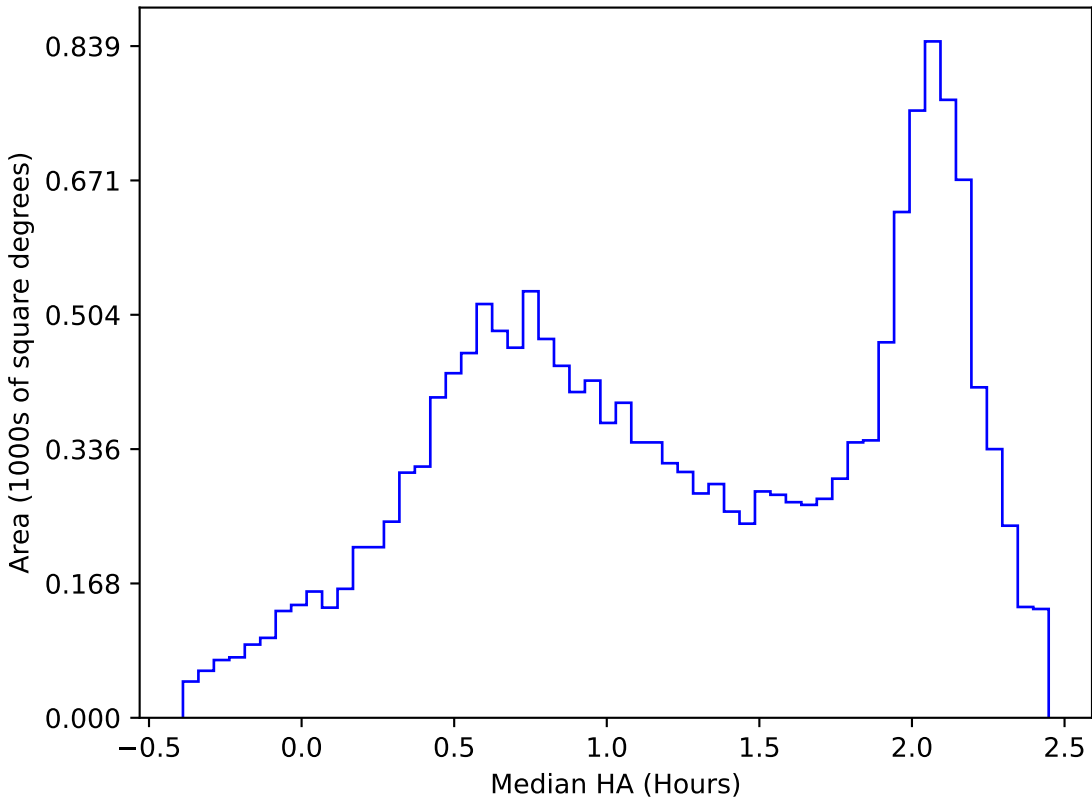
internal_u_expt30_nscale1.5v3.4_10yrs WFD y band: Median HA
